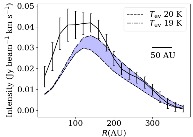
Fig. 1: The black continuous line shows the observed DCO + radial profile. These profiles are obtained by averaging the values of concentric ellipsoids of the integrated intensity maps. The error bars of the observed DCO + radial profile corresponds to 3\sigma , where \sigma is the standard deviation of the values contained in the ellipsoid divided by the square root of the number of beams. The 50 AU bar corresponds to the semi-minor axis of the synthesized beam and serves as a measure of the spatial resolution. The dashed lines show radial profiles of the emission from models with two different evaporation temperature of CO T_{\text{CO}}=19\text{-}20 K and a constant abundance X_{\text{in}}=5.0\times 10^{-5}
