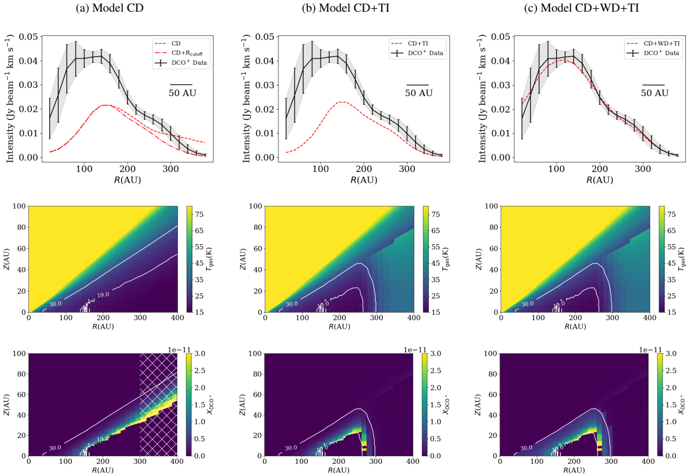
Fig. 4: The top panels show the resulting radial profile of the DCO + integrated intensity map of both models and data. The error bars on the data corresponds to 3\sigma , where \sigma is calculated as the standard deviation of a single ellipsoid divided by the square root of the number of beams. The middle panels show the models' temperature profile with contours at 19 and 30 K. The bottom panel shows the DCO + abundance profile over-plotted with temperature contours at 19 and 30 K. The hatched region in the DCO + abundance from model CD marks the radial cut off used in our standard model to reproduce the absence of emission at R > 300 AU.
