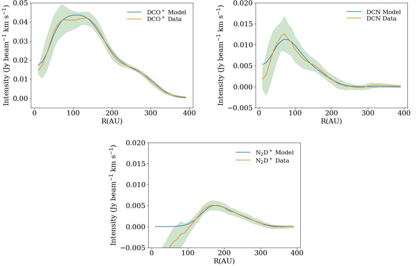
Fig. 6: Best-fit models for the transitions of \text{DCO}^+ J=3-2 , \text{DCN} J=3-2 , and \text{N}_2\text{D}^+ J=3-2 . The error bars, shown as a filled region in green, correspond to the standard deviation of the values in one annulus as seen in Fig. 3.
