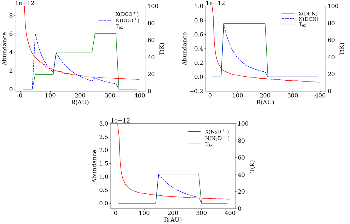
Fig. 5: Schematics of the abundance models for the transitions of \text{DCO}^+ J=3-2 , \text{DCN} J=3-2 and \text{N}_2\text{D}^+ J=3-2 . The dashed blue line corresponds to a scaled profile of the column density of the abundance model for the purpose of illustration. The red continuous line corresponds to the assumed excitation temperature profile.
