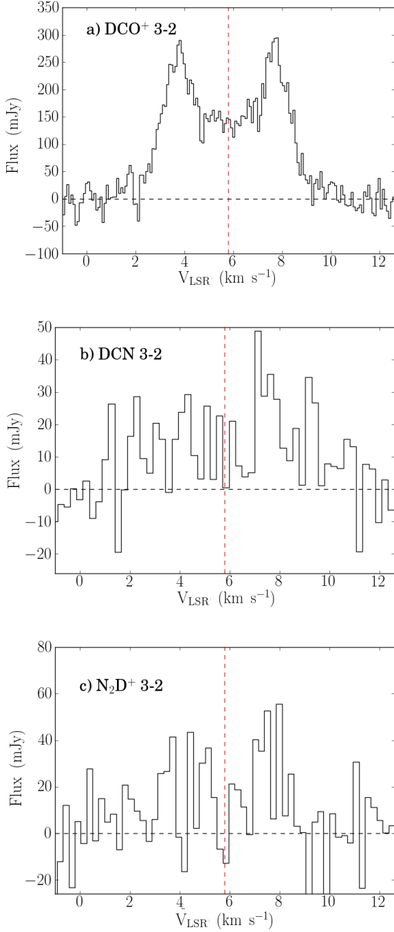
Fig. 2: Spectra of a) \text{DCO}^+ J=3-2 , b) \text{DCN} J=3-2 , and c) \text{N}_2\text{D}^+ J=3-2 of the disk integrated values using a Keplerian mask as shown in Fig. 1. The \text{DCN} and \text{N}_2\text{D}^+ spectra have been binned to 3 times their resolution, 0.255 km/s and 0.238 km/s, respectively, to enhance their S/N ratio.
