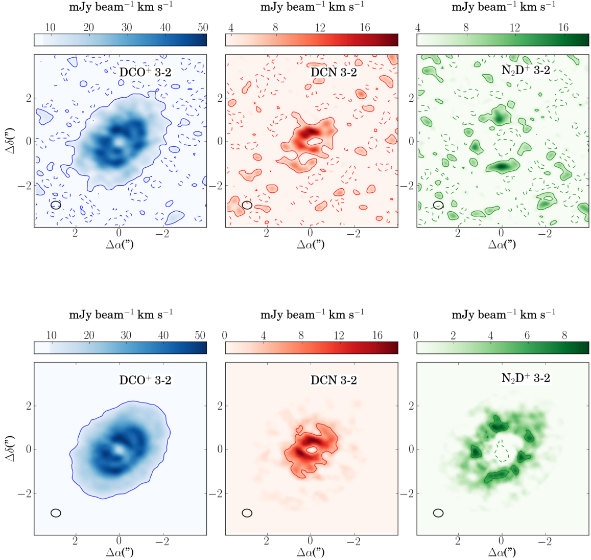
Fig. 1: Integrated intensity maps of \text{DCO}^+ , \text{N}_2\text{D}^+ , and \text{DCN} with (lower panels) and without (upper panels) a Keplerian mask as explained in Appendix A. The resulting synthesized beams of 0''.53 \times 0''.42 for \text{DCO}^+ and \text{DCN} , and 0''.50 \times 0''.39 for \text{N}_2\text{D}^+ using natural weighting are shown at the lower left of each map. Contours are 1\sigma levels, where \sigma is estimated as the rms of an emission free region in the sky.
