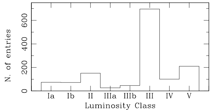
Fig. 7. Distribution of luminosity class.
