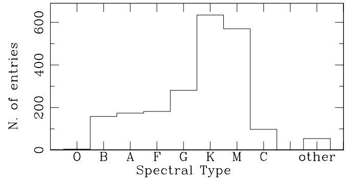
Fig. 6. Distribution of spectral type.
