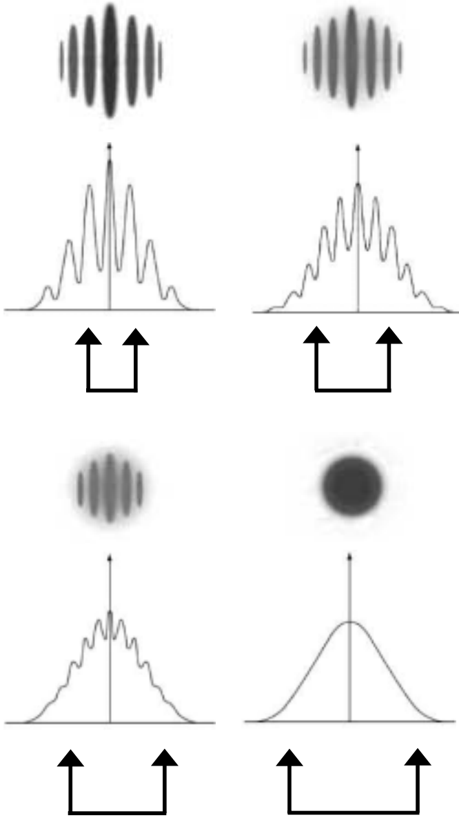
Fig. 2. Interference fringes on a stellar object are shown at different baselines. When the baseline between the two telescopes increases, the contrast of the fringes decreases. At a given baseline the fringes disappear. The diameter (or spatial parameters) of the object can be extracted from these data.
