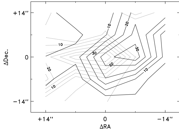
Fig. 3. Contour map of the wing CO J = 6 \rightarrow 5 emission toward EL 29. The solid lines show the blue shifted emission integrated between -10 and 0 \text{ km s}^{-1} , while the dotted lines show the red shifted emission in the interval +7 to +17 \text{ km s}^{-1} . Levels of 5, 10, 15, 20, 25, and 30 \text{ K km s}^{-1} are shown.
