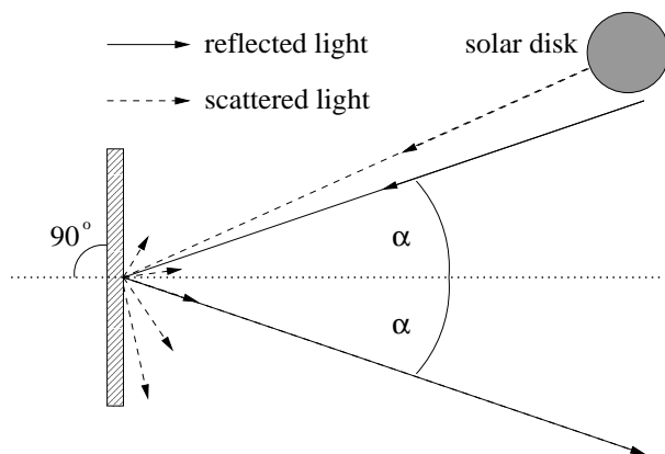
FIGURE 14. Light paths for obliquely reflected (from above the solar limb) and scattered light (from all over the solar disk) on a flat mirror. Note that scattered light does not follow the rule of equal angles of incidence for the incoming and outgoing beams. Part of the scattered light goes in the same direction as the reflected light, thus contributing to the measured signal.
