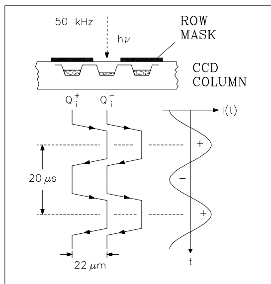
FIGURE 21. Principle of the ZIMPOL I CCD demodulator. A cross section through a part of the CCD sensor is shown at the top. The motion of the charge packets in the CCD are shown as a function of the modulation indicated in the right.
