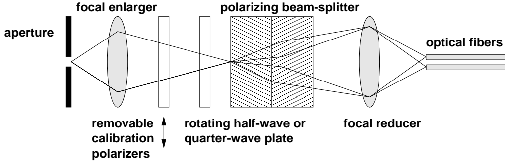
FIGURE 20. Optical layout of the MuSiCoS polarimeter by Donati et al. (1999). An entrance aperture provides a fixed field of view independent of seeing. A focal enlarger provides a slow beam through the polarimeter to avoid large angles of inclination on the polarization optics. Circular and linear polarizers can be inserted to calibrate the polarimeter. A rotating quarter-wave or half-wave plate provides the beam exchange. A polarizing beam-splitter splits the beam into two opposite polarization states that are reimaged onto the ends of two fibers that lead to the echelle spectrograph.
