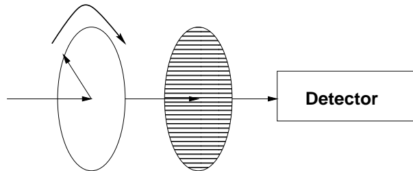
FIGURE 3. A simple polarimeter consisting of a rotating retarder and a fixed linear polarizer, which together make up the modulator package. The arrow on the retarder indicates the orientation of the fast axis (see below).
