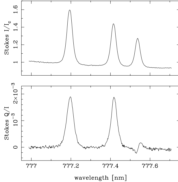
FIGURE 15. True scattering polarization in the OI triplet at 777 nm about 1'' above the limb. The polarization of the continuum has been set to zero because the observations do not allow a correct measurement of the continuum polarization.
