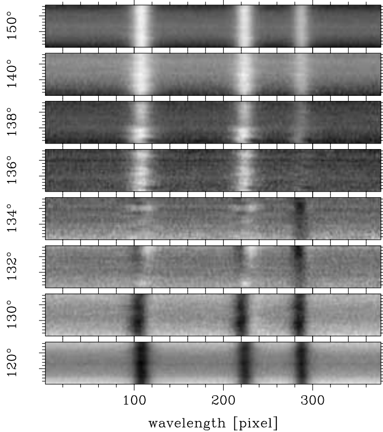
FIGURE 13. Observed Stokes Q/I signal in the OI 777 nm triplet about 1'' above the limb as a function of position angle, measured clockwise from geographic north. Lighter-than-average shading denotes polarization along the limb and darker-than-average shading denotes polarization perpendicular to the limb.
