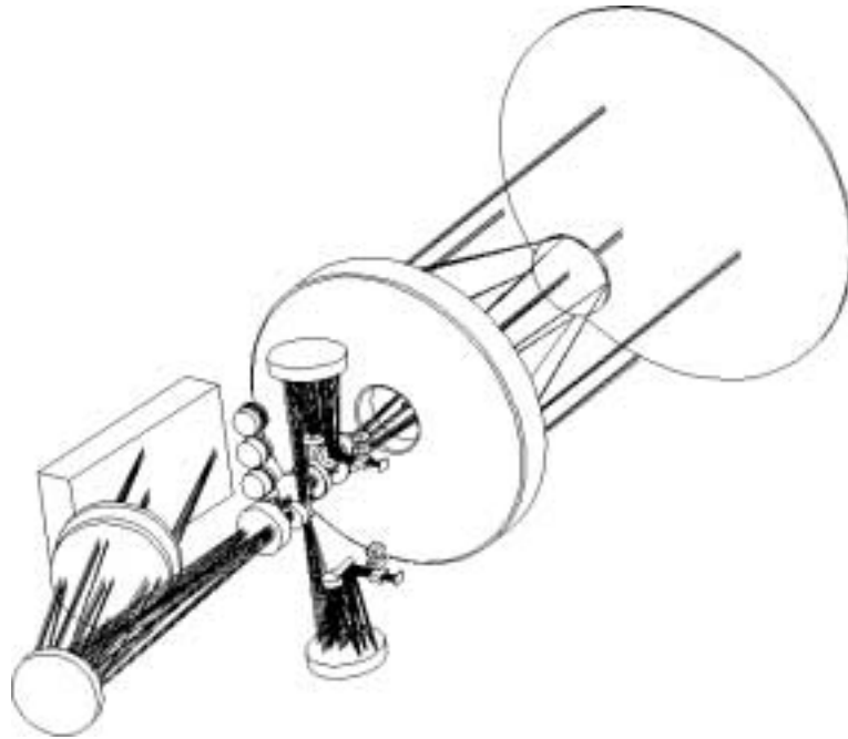
FIGURE 27. The optical layout of the SOLIS Vector-Spectromagnetograph. The entrance window is on the upper right, and the folded Littrow spectrograph is on the lower left side of the drawing.
