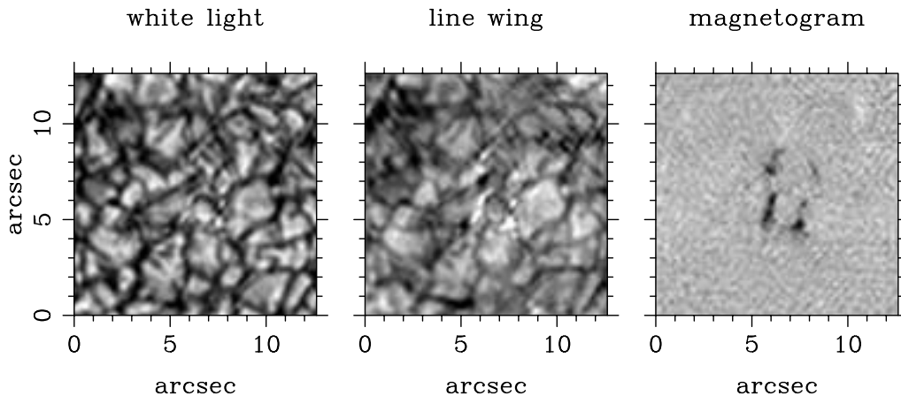
FIGURE 24. An example of a high-resolution observation of solar network magnetic fields close to disk center in Cal 610.3 nm using ZIMPOL I and speckle polarimetry to remove the effects of seeing. The magnetic fields are concentrated in very small areas and tend to be bright in both the white-light and the line-wing images.
