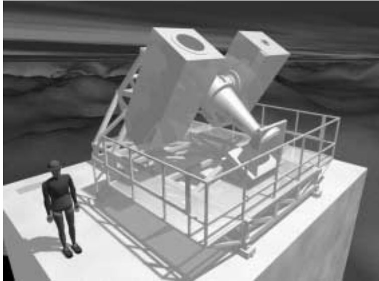
FIGURE 26. Artists impression of SOLIS on top of the Kitt Peak Vacuum Telescope building. The instrument with the large entrance window is the Vector-Spectromagnetograph.
