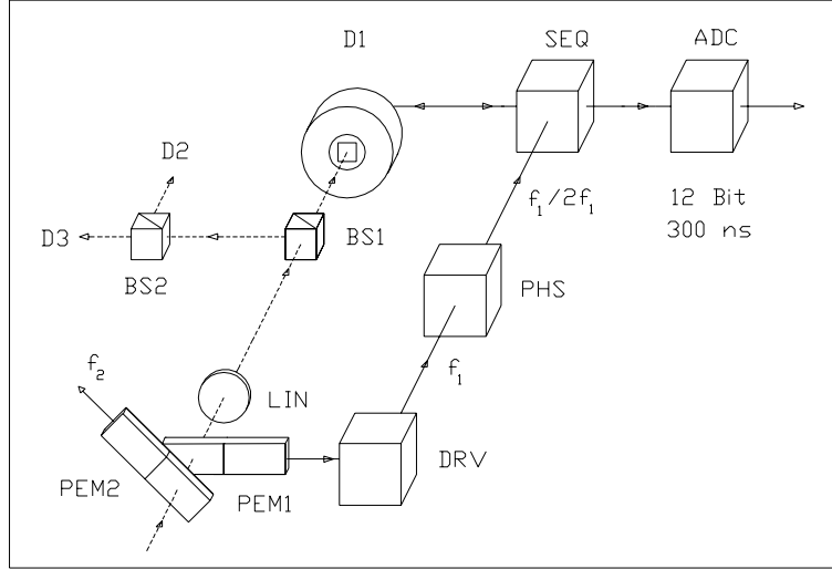
FIGURE 22. Setup for recording all four Stokes parameters with two photoelastic modulators. The orientation of the components is given with respect to Stokes Q . PEM1 ( 0^\circ ), PEM2 ( 45^\circ ): photoelastic modulators, LIN ( 22.5^\circ ): Glan linear polarizer, BS1, BS2: beam splitter cubes that direct the modulated light to detectors D1, D2, and D3.
