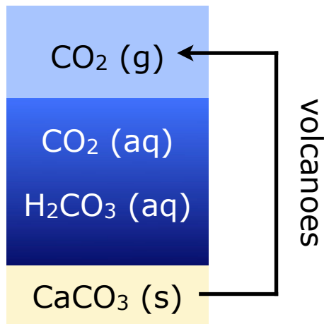
CO 2 is stored in the famous lime stone cliffs in Dover
