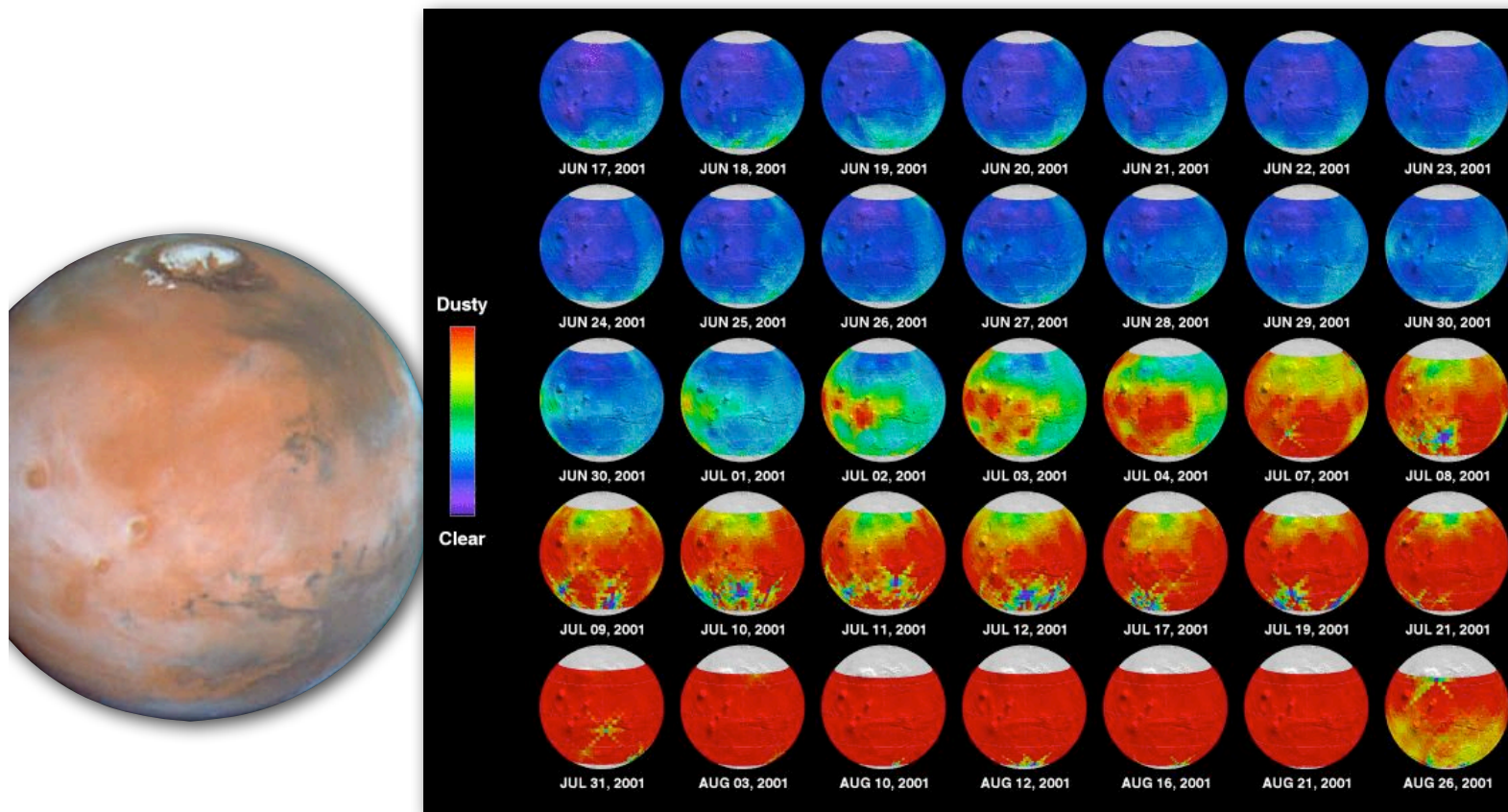
Thermal Emission Spectrometer (TES, MGS) observations
