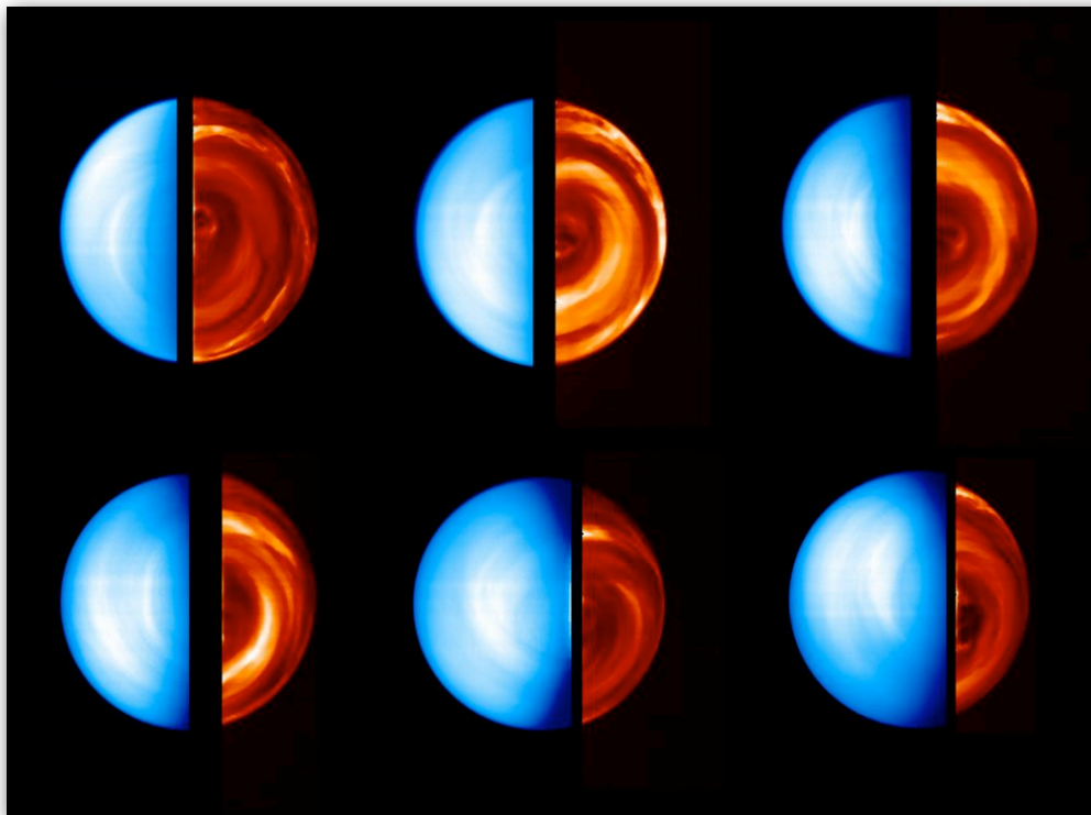
Bright @ 1.7 \mu\text{m} : low, warm clouds; Dark @ 1.7 \mu\text{m} : upper, cold clouds; VIRTIS/VEX/ESA
