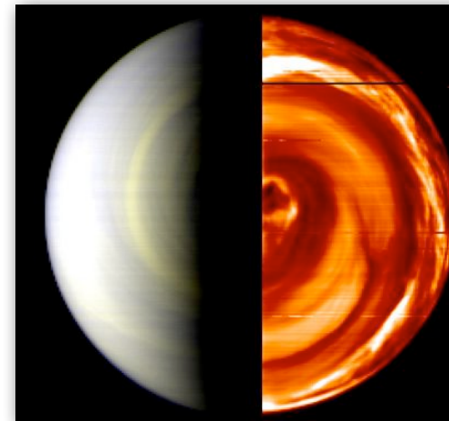
Venus' day and night side (VIRTIS, Venus Express, ESA)
