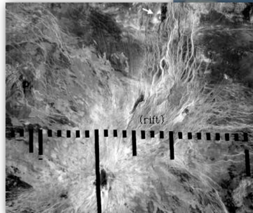
Venus: Theia Mons, 4 km altitude
