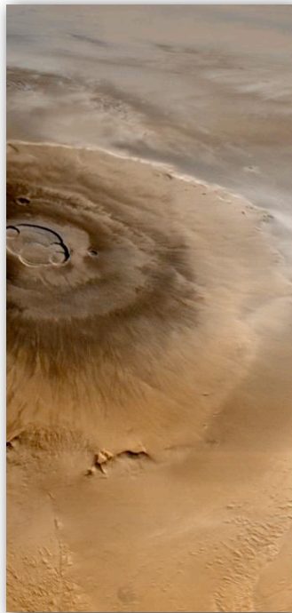
Mars: Olympus Mons, 25 km of altitude
