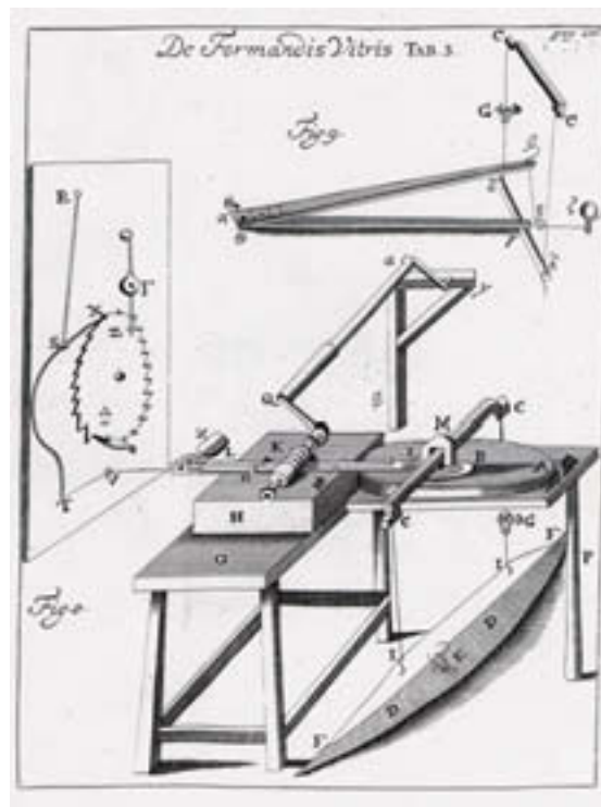
Figure 2: Lens-grinding machine of Christiaan Huygens (From his 'Opuscula Posthuma', published posthumously by Janssionio Waesbergios, Amsterdam, 1728 )
