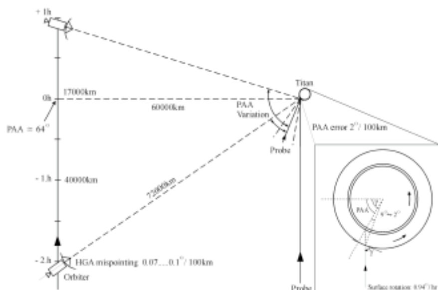
Figure 5: Orbiter Trajectory during the Probe mission
