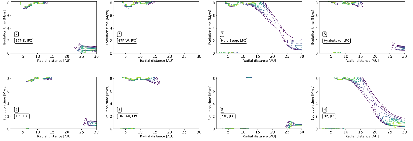
Fig. 4. Maximum likelihood surfaces for the reset scenario, considering C and O bearing species only. Radius in AU in the physically evolving protoplanetary disk midplane is on the x -axis, and evolution time in Myrs is on the y -axis.
