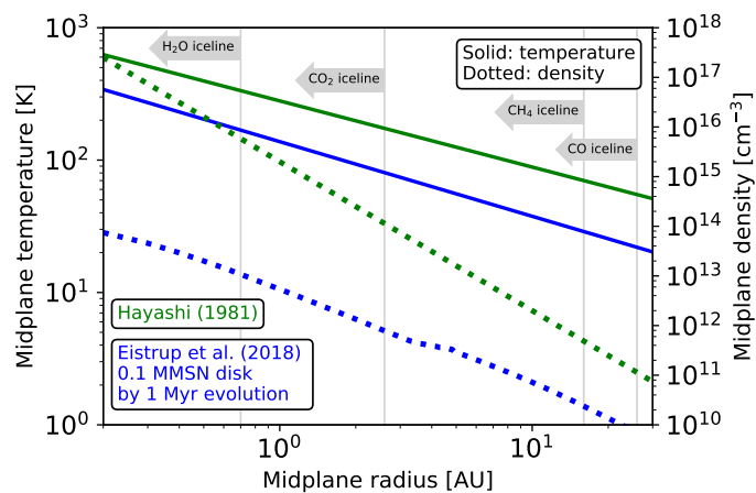
Fig. 1. Physical structures of the disk midplanes for the pre-Solar nebula from Hayashi (1981) (in green), and for the 0.1 MMSN disk by 1 Myr evolution from Eistrup et al. (2018) (in blue). Solid profiles are for temperature. Dotted profiles are for number density. The vertical grey lines indicate the positions of the icelines of \text{H}_2\text{O} , \text{CO}_2 , \text{CH}_4 and \text{CO} by 1 Myr evolution for the 0.1 MMSN disk in Eistrup et al. (2018). The grey arrows on each of the vertical lines indicate which species each line is associated with, and how the iceline moves over time (all inwards).
