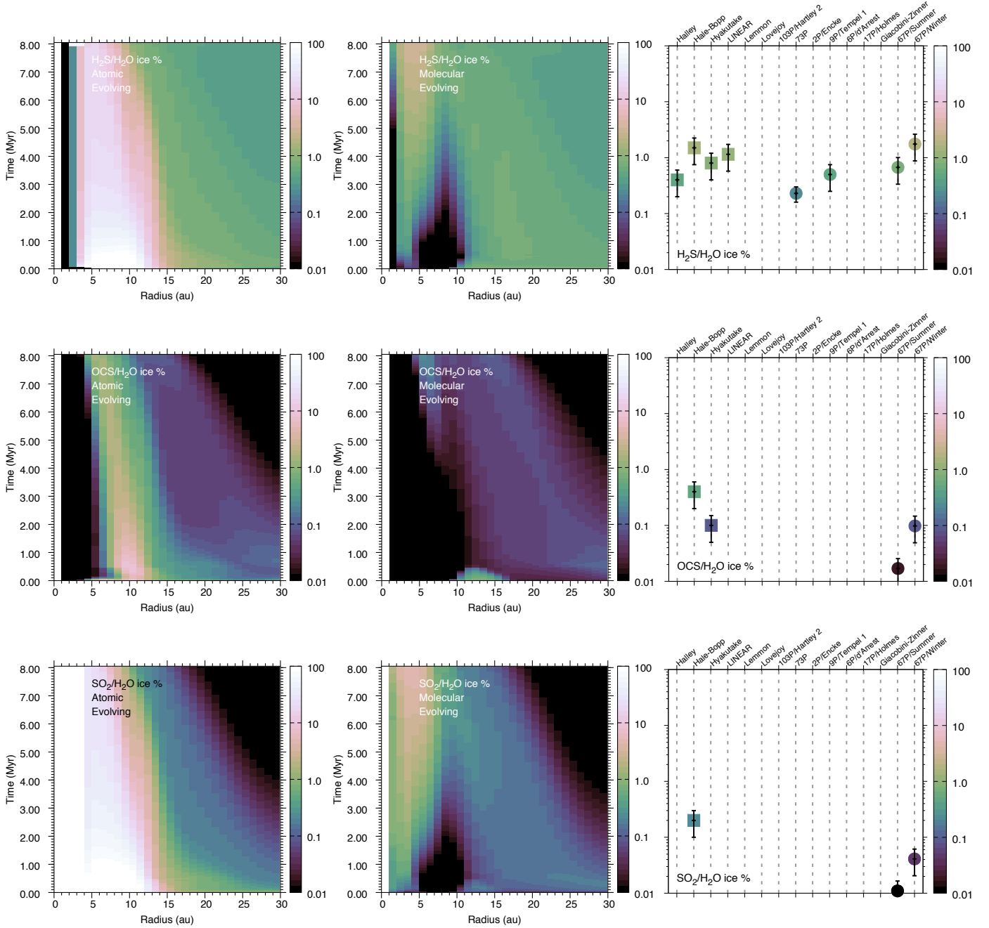
Fig. A.4. Same as Figure A.1 for \text{H}_2\text{S} , OCS, and \text{SO}_2 ice.
