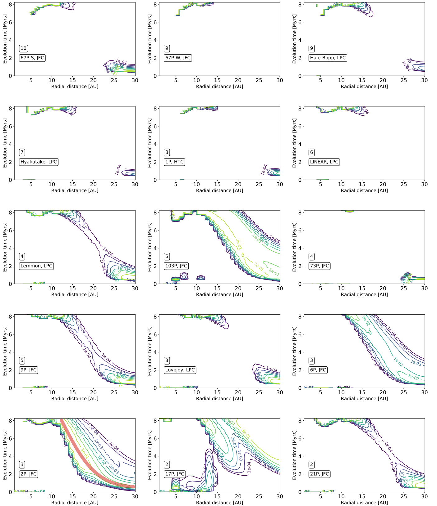
Fig. 2. Maximum likelihood surfaces for the reset scenario, for the full sample of molecular species. Radius in AU in the physically evolving protoplanetary disk midplane is on the x -axis, and evolution time in Myrs is on the y -axis. The red shaded region for comet 2P indicates the trail through parameter space (largely tracing the vicinity of the CO iceline) on which most of the comets show good agreement with formation.
