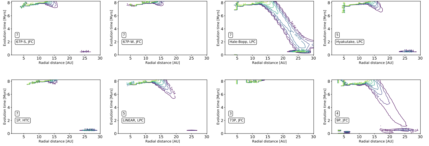
Fig. 5. Maximum likelihood surfaces for the inheritance scenario, considering C and O bearing species only. Radius in AU in the physically evolving protoplanetary disk midplane is on the x -axis, and evolution time in Myrs is on the y -axis.
