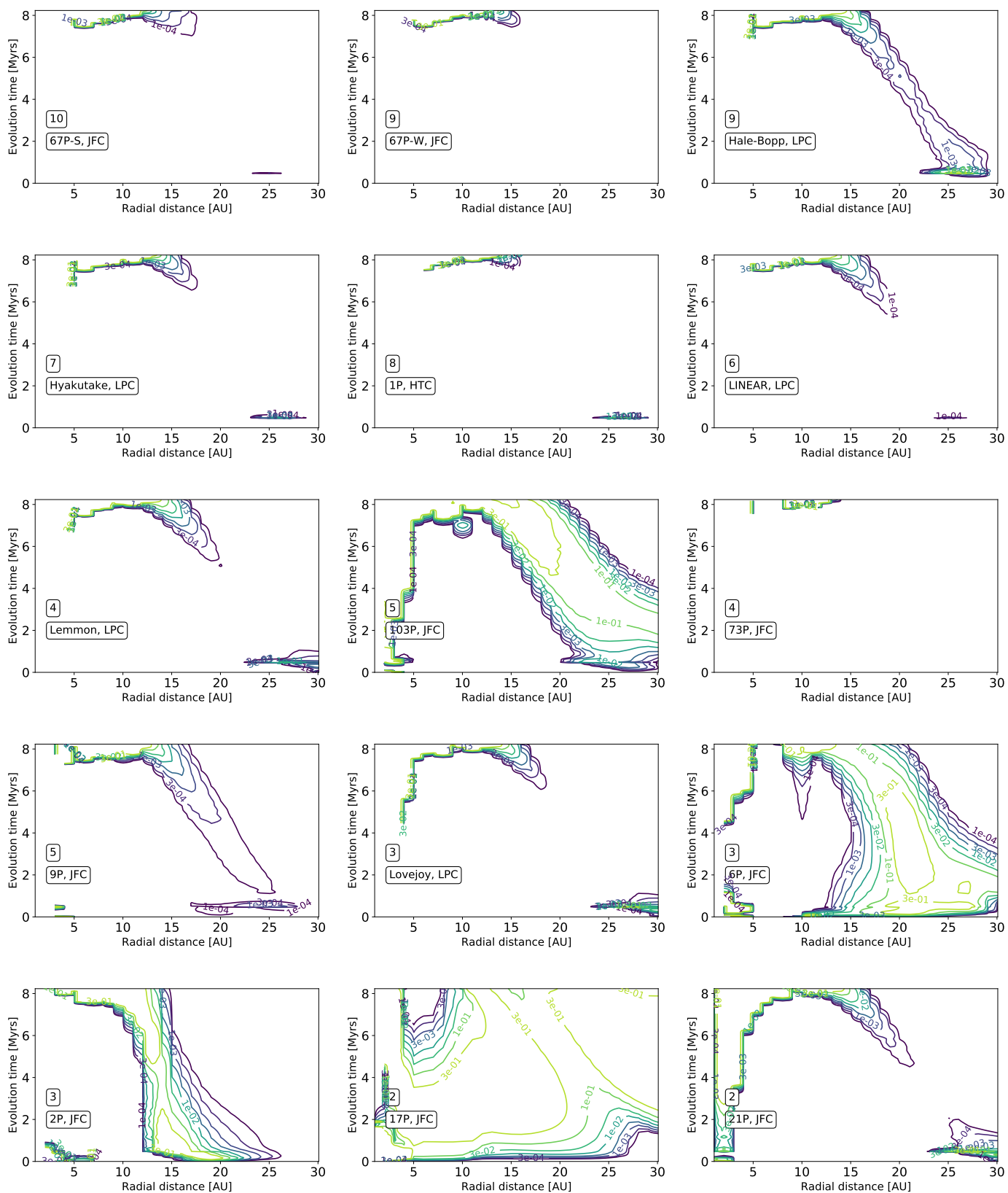
Fig. 3. Maximum likelihood surfaces for the inheritance scenario, for the full sample of molecular species. Radius in AU in the physically evolving protoplanetary disk midplane is on the x -axis, and evolution time in Myrs is on the y -axis.
