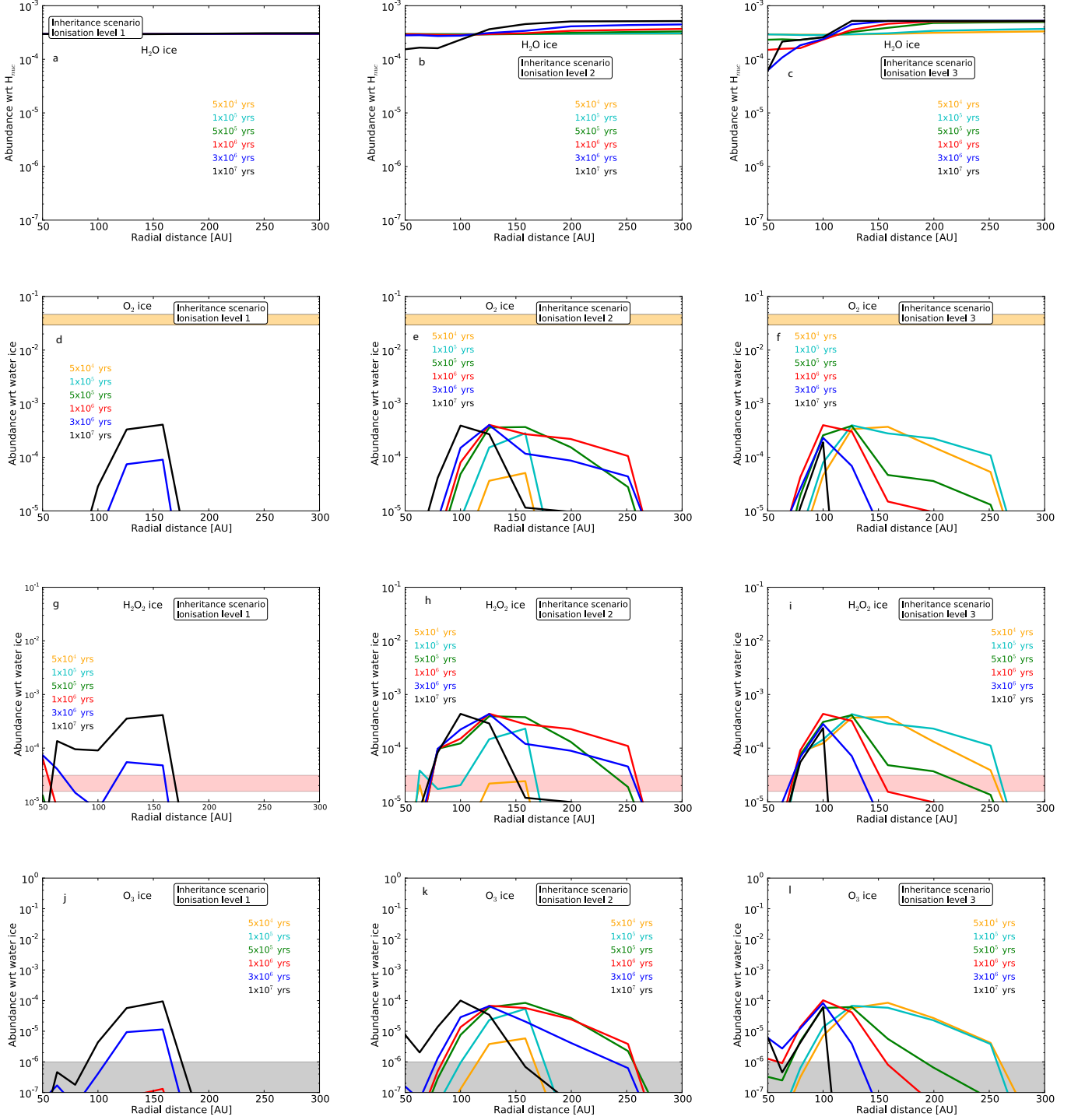
Fig. 5: Radial abundances profiles, for the inheritance scenario at multiple evolutionary time steps. Top to bottom are H 2 O, O 2 and H 2 O 2 and O 3 ices. Left to right are increasing ionisation levels. For O 2 , H 2 O 2 , and O 3 the limits, and upper limit, detected in comet 67P, are indicated as yellow, red and grey shaded areas, respectively. The chemical network utilised includes O 3 chemistry.
