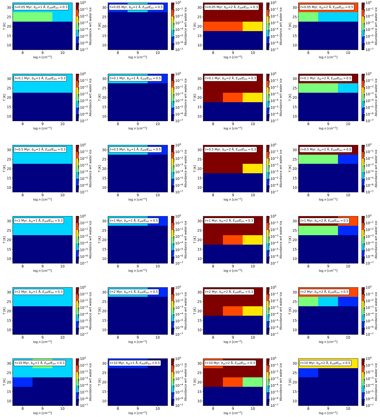
Fig. A.5: Abundances (given as colors) for \text{H}_2\text{O}_2 ice as function of midplane density ( x -axes), and temperature ( y -axes) at different evolutionary steps for the reset scenario. From left to right are abundances from model runs with different parameters for grain-surface reactions: columns one and two feature b_{qt} = 1 \text{ \AA} , columns three and four feature b_{qt} = 2 \text{ \AA} , columns one and three are with E_{\text{diff}}/E_{\text{bin}} = 0.3 , and columns two and four are with E_{\text{diff}}/E_{\text{bin}} = 0.5 . Top to bottom are different evolutionary times, from 0.05 Myr (top) to 10 Myr (bottom). To the right of each plot is a colorbar, indicating the abundance level with respect to \text{H}_2\text{O} ice for each color. The chemical network utilised includes \text{O}_3 chemistry. Lightest hue of blue matches the cometary \text{H}_2\text{O}_2 abundances.
