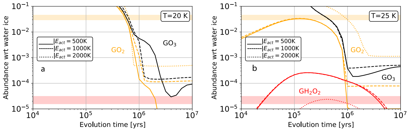
Fig. 10: Evolving abundances for O 2 ice, H 2 O 2 ice and O 3 ice for three different activation energies for the reaction i\text{O} + i\text{O}_2 . a) is for T=20 K. b) is for T=25 K. The barrier width for quantum tunnelling is b_{qt} = 2 \text{ \AA} , and the molecular diffusion-to-binding energy is 0.5.
