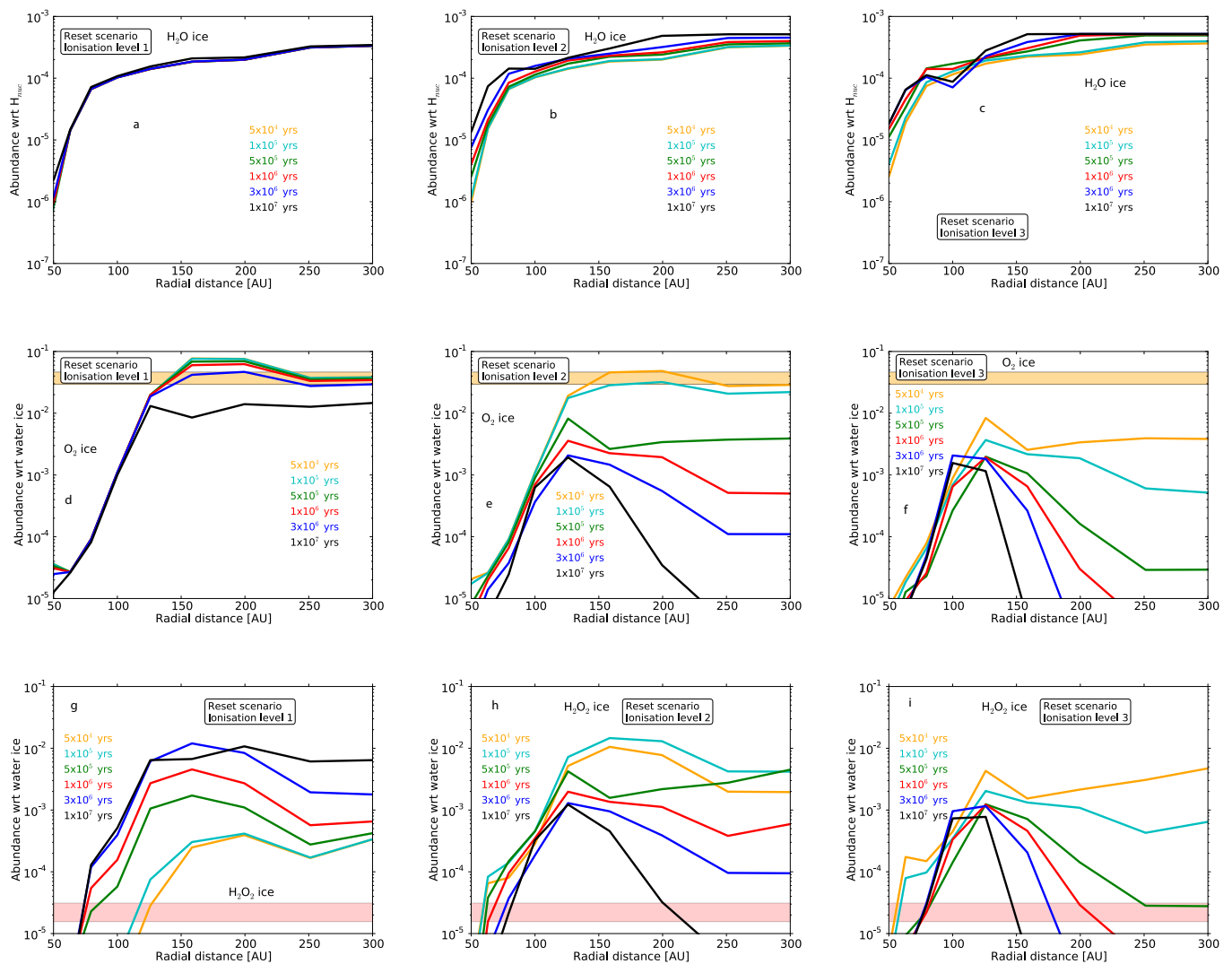
Fig. 3: Radial abundances profiles, for the reset scenario at multiple evolutionary time steps. Top to bottom are H 2 O, O 2 and H 2 O 2 ices. Left to right are increasing ionisation levels. For O 2 and H 2 O 2 the limits detected in comet 67P are indicated as yellow and red shaded area, respectively. The chemical network utilised does not including O 3 chemistry.
