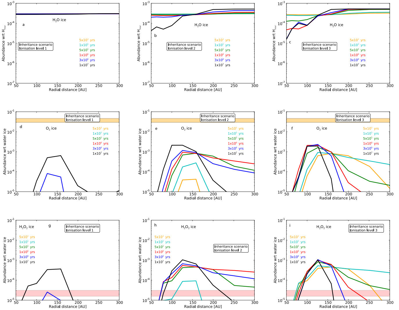
Fig. 2: Radial abundances profiles, for the inheritance scenario at multiple evolutionary time steps. Top to bottom are H 2 O, O 2 and H 2 O 2 . Left to right are increasing ionisation levels. For O 2 and H 2 O 2 the limits detected in comet 67P are indicated as yellow and red shaded area, respectively. The chemical network utilised does not including O 3 chemistry.
