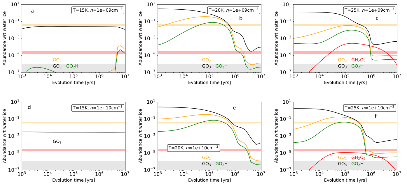
Fig. 9: Evolving abundances as function of time for the reset scenario six different combinations of temperature (15, 20 or 25 K), density ( 10^9 or 10^{10} \text{cm}^{-3} ) and molecular diffusion-to-binding energy of 0.5. The barrier width for quantum tunnelling is b_{qt} = 2 \text{ \AA} . The orange shaded regions indicates the limits to the measured abundance of O 2 ice in the coma of comet 67P. The red shaded regions indicates the limits to the measured abundance of H 2 O 2 , and the top of the grey shaded region marks the upper limit to the measured abundance of O 3 ice in comet 67P. The chemical network utilised includes O 3 chemistry.
