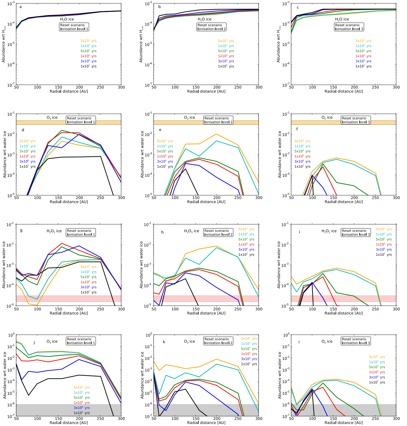
Fig. 6: Radial abundances profiles, for the reset scenario at multiple evolutionary time steps. Top to bottom are H 2 O, O 2 and H 2 O 2 and O 3 ices. Left to right are increasing ionisation levels. For O 2 , H 2 O 2 , and O 3 the limits, and upper limit, detected in comet 67P, are indicated as yellow, red and grey shaded areas, respectively. The chemical network utilised includes O 3 chemistry.
