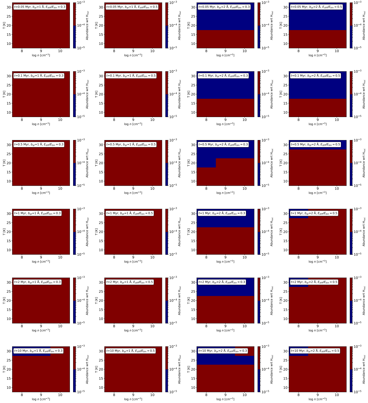
Fig. A.3: Abundances (given as colors) for \text{H}_2\text{O} ice as function of midplane density ( x -axes), and temperature ( y -axes) at different evolutionary steps for the reset scenario. From left to right are abundances from model runs with different parameters for grain-surface reactions: columns one and two feature b_{qt} = 1 \text{ \AA} , columns three and four feature b_{qt} = 2 \text{ \AA} , columns one and three are with E_{\text{diff}}/E_{\text{bin}} = 0.3 , and columns two and four are with E_{\text{diff}}/E_{\text{bin}} = 0.5 . Top to bottom are different evolutionary times, from 0.05 Myr (top) to 10 Myr (bottom). To the right of each plot is a colorbar, indicating the abundance level with respect to \text{H}_{\text{nuc}} for each color. The chemical network utilised includes \text{O}_3 chemistry.
