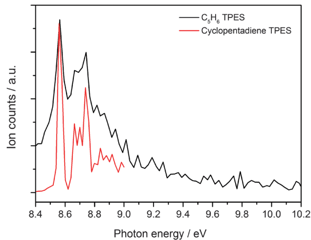
Fig. 3 Mass selected threshold photoelectron spectrum of C_5H_6 formed in the reaction between C_3H_5^* and C_2H_2 (in black) plotted together with a measured spectrum of cyclopentadiene (in red).
