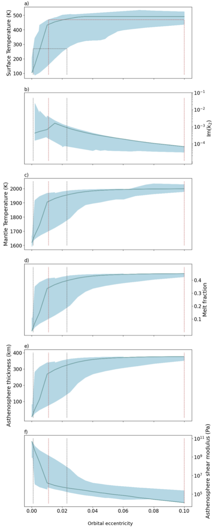
Fig. 11. Computed ranges for the model’s output parameters (Table 3) that lead to exo-Ios with a = 4.65 Roche radii and a radius of 2 \times R_{Io} in a stable thermal equilibrium. The blue line corresponds to the nominal values analysis (Sect. 5). The gray and red dotted lines respectively show the limits of a 270 K and 470 K surface temperature observation.
