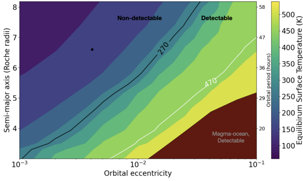
Fig. 6. Surface equilibrium temperature of a 2R_{\text{Io}} THEM as a function of its orbital eccentricity ( e ) and semi-major axis ( a ). The black dot indicates Io’s current orbital parameters. The nominal values of the interior parameters that we used are presented in Table 2. The 270 K isotherm divides the parameter space into detectable and non-detectable exomoons.
