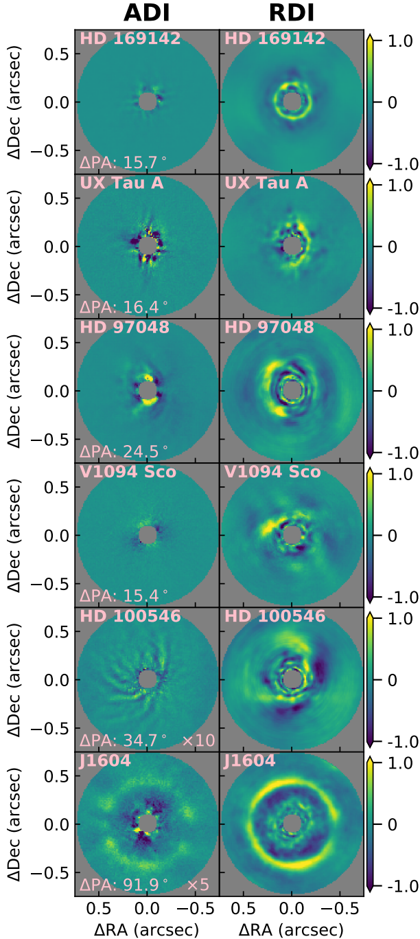
Fig. 8. Comparison of SPHERE/IRDIS disk images in H_{23} reduced with ADI (left) and RDI (right). An arbitrary linear color scale is applied, which is normalized to the maximum flux in the RDI image of each target. Because the ADI images of HD 100546 and J1604 severely suffer from flux loss due to self-subtraction, we linearly scaled these ADI images by factors of 10 and 5, respectively. The star is located in the center of each image. The central gray region shows the position of the coronagraph mask with a diameter of 196 mas (16 pixels). The adopted FoV is 0.735'' in radius.
