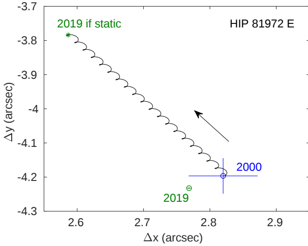
Fig. 14. Proper motion test for the “E” candidate around HIP 81972. The black arrow denotes the direction of time for background motion. For this case, the candidate is consistent with CPM, while simultaneously being clearly distinct from the static background location. It is a probable physical companion.
