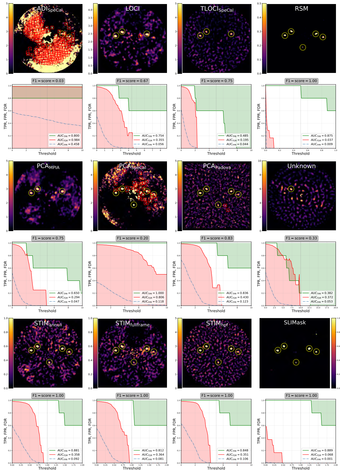
Figure 2. Results of the ADI subchallenge for the sph3 VLT/SPHERE-IRDIS dataset: speckle subtraction techniques.
