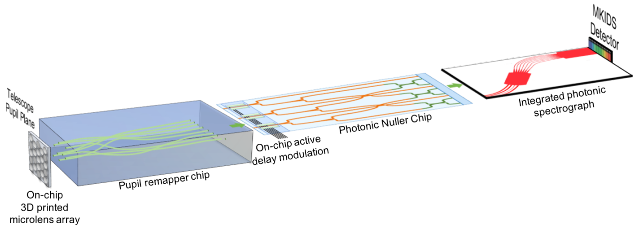
Figure 10. Conceptual sketch for an ultimate photonic instrument for high-contrast imaging. [ N. Jovanovic, B. Norris, N. Cvetojevic ]
