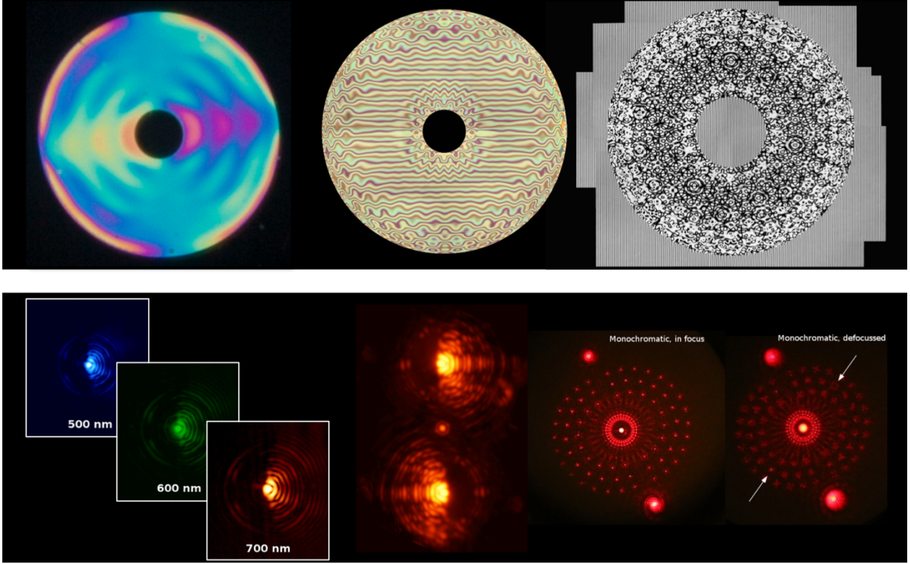
Figure 4. Top : stitched microscope images of vector-APP devices in between crossed polarizers. 23–25 Bottom : Vector-APP point-spread functions. The first and the third correspond to the pupil phase patterns above. The middle one is an on-sky result from Ref. 26 .
