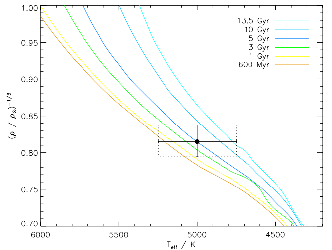
Figure 8. Modified Hertzsprung–Russell diagram comparing the effective temperature and light-curve stellar density for WTS-2, with the PARSEC v1.0 stellar evolution isochrones (Bressan et al. 2012) for Z = 0.019 . The data point and its error box marks the allowed values for WTS-2. Assuming the star is not on the pre-main sequence, the isochrones give an age constraint of >600 Myr.
