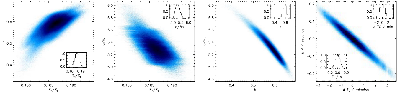
Figure 9. Distributions of correlated parameters in the MCMC analysis of the dilution-corrected light curves. The insets show individual parameter (normalized) histograms to highlight the skew in the distributions.
