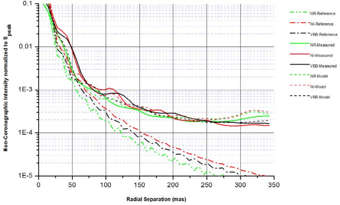
Figure 9 Measured non-coronagraph intensity profiles normalized to S_{\text{peak}} under atmospheric turbulent conditions (0.85 asec seeing and 10 m/s windspeed) for filters NR, NI and VBB. The calculated Airy patterns for each filter are shown for reference. Also shown are the model predictions from the CAOS simulations.
