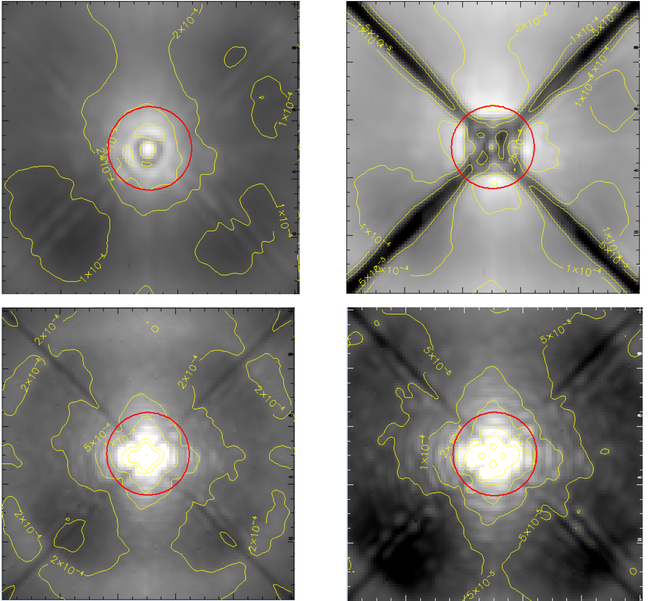
Figure 10 Coronagraphic intensity images under atmospheric turbulent conditions (0.85 asec seeing and 10 m/s windspeed) for coronagraphs 3 \lambda/D -VBB (top left), 5 \lambda/D – VBB (top right), 4QPM1 – NR (bottom left) and 4QPM2 – NI (bottom right). The images are normalized to Speak. The display scaling for 4QPM1&2 is set to saturate the core to enhance the features in the outer regions. The radius of the circle is 100 mas.
